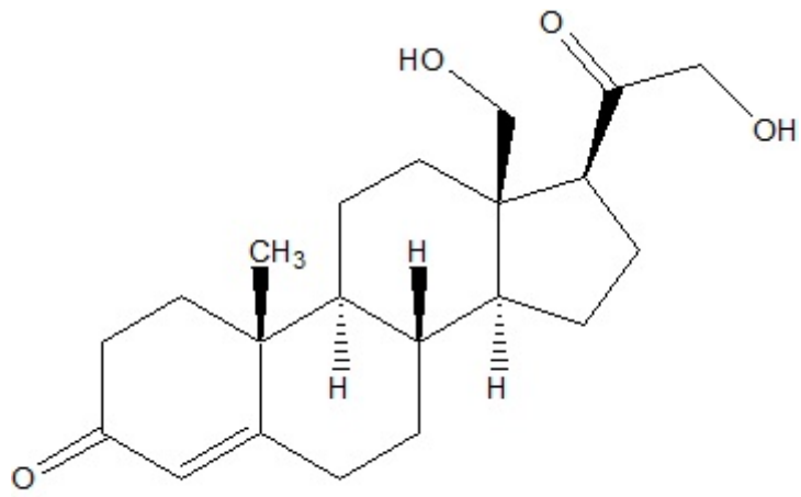
18-Hydroxy-11-deoxycorticosterone
