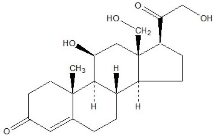
18-Hydroxycorticosterone
